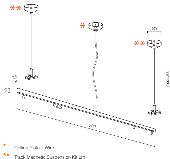
52M2034WH-AZ4821 track magnetic 2m, 3000K, white
